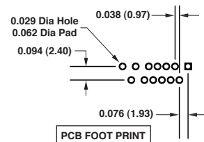
PCB FOOTPRINT
