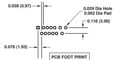
PCB FOOTPRINT
