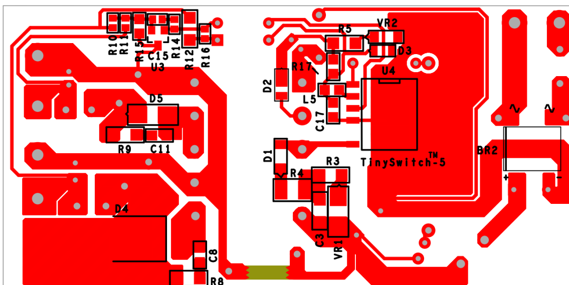
Figure 5 – Printed Circuit Board, Bottom View.
