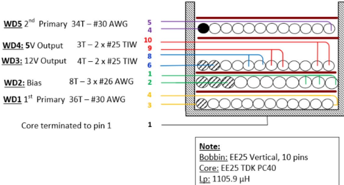
Figure 7 – Transformer Build Diagram.
