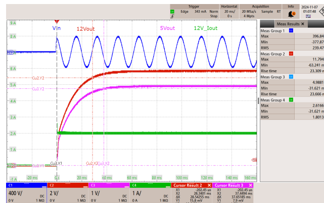
Figure 76 – 265 VAC 50 Hz.
