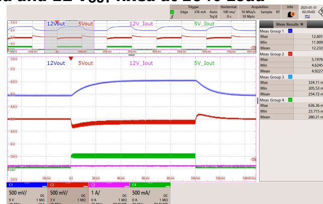
Figure 86 – 115 VAC 60 Hz.
