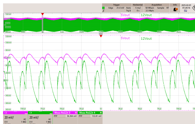
Figure 106 – 265 VAC 50 Hz.
