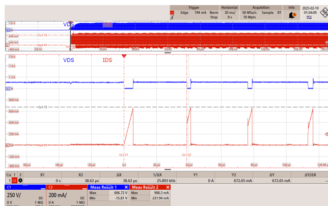
Figure 35 – 230 VAC 50 Hz.
