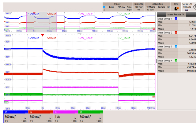
Figure 98 – 115 VAC 60 Hz.
