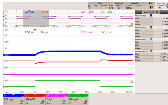
Figure 92 – 265 VAC 50 Hz.
