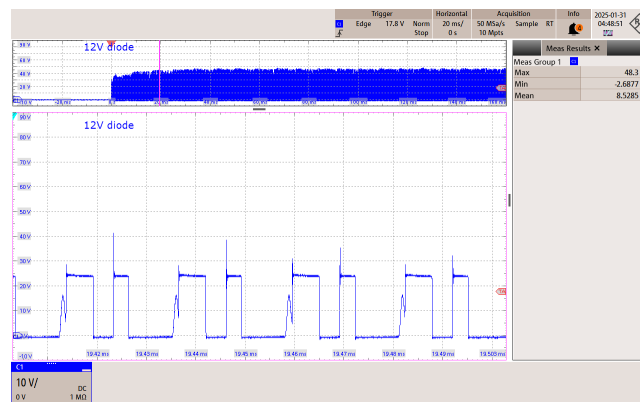
Figure 50 – 115 VAC 60 Hz.
