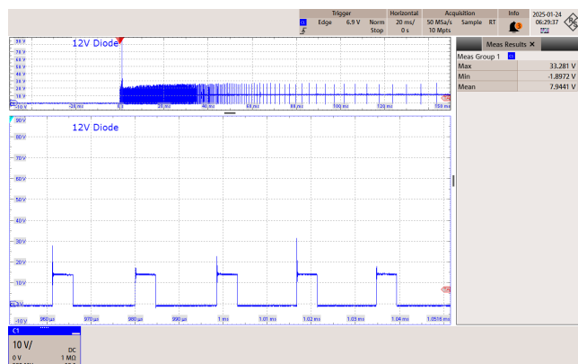
Figure 53 – 85 VAC 60 Hz.
