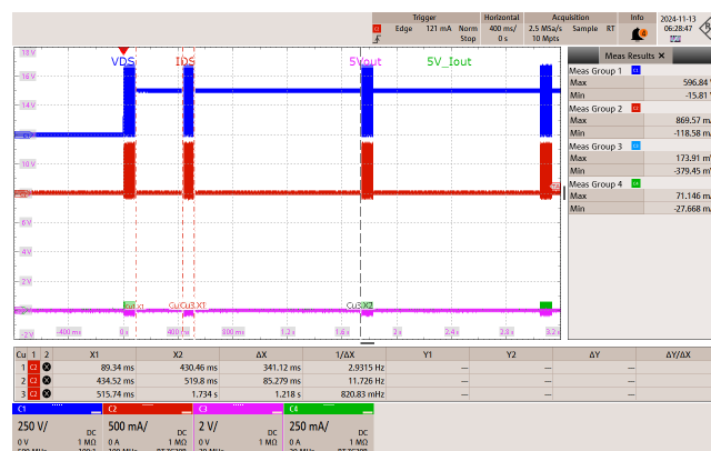
Figure 132 – 265 VAC 50 Hz 5 V Start-Up Output Short.
