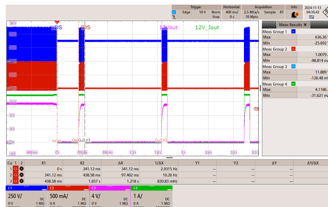
Figure 138 – 265 VAC 60 Hz. 12 V / 3.5 A, 5 V / 0.875 A.
