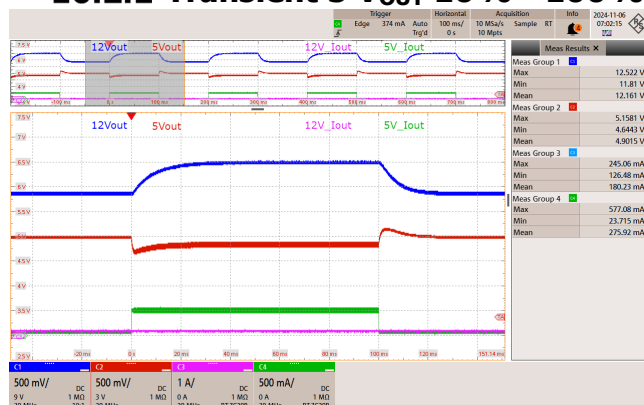
Figure 85 – 85 VAC 60 Hz.
