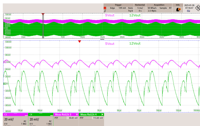
Figure 105 – 230 VAC 50 Hz.
