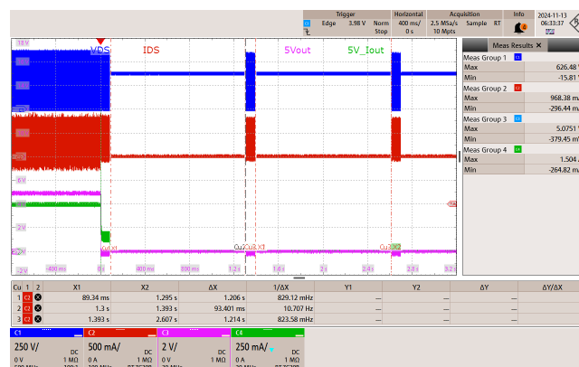
Figure 136 – 265 VAC 50 Hz 5 V Running Output Short.
