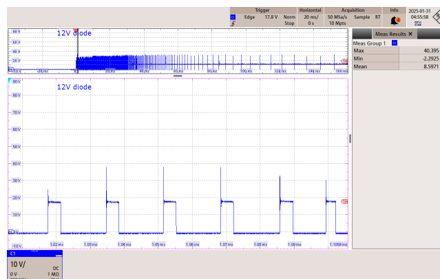
Figure 54 – 115 VAC 60 Hz.
