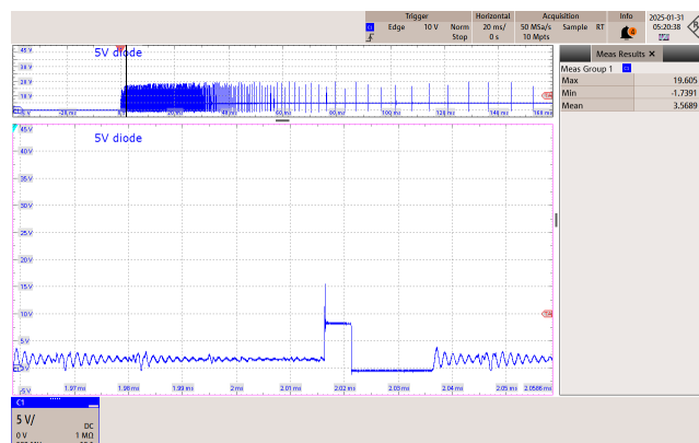
Figure 70 – 115 VAC 60 Hz.
