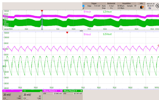
Figure 103 – 85 VAC 60 Hz.
