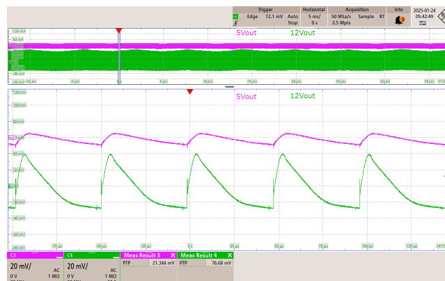
Figure 118 – 265 VAC 50 Hz.
