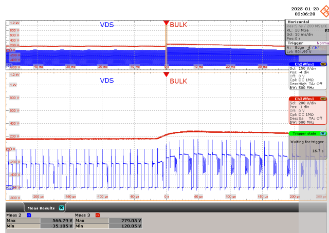
Figure 146 – 115 VAC 60 Hz +1kV_90°
