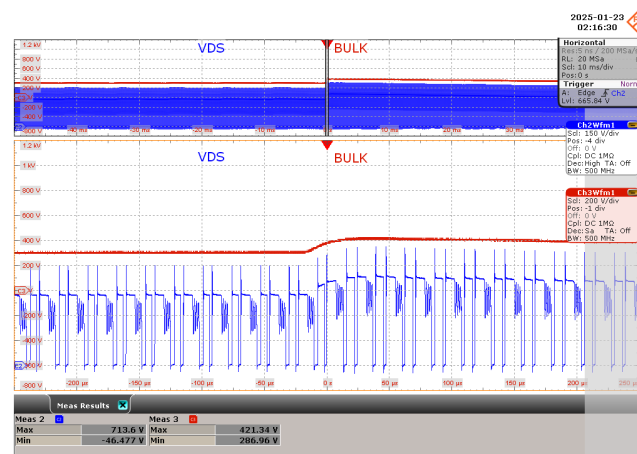
Figure 147 – 230 VAC 60 Hz +1kV_90°
