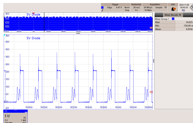
Figure 60 – 265 VAC 50 Hz.
