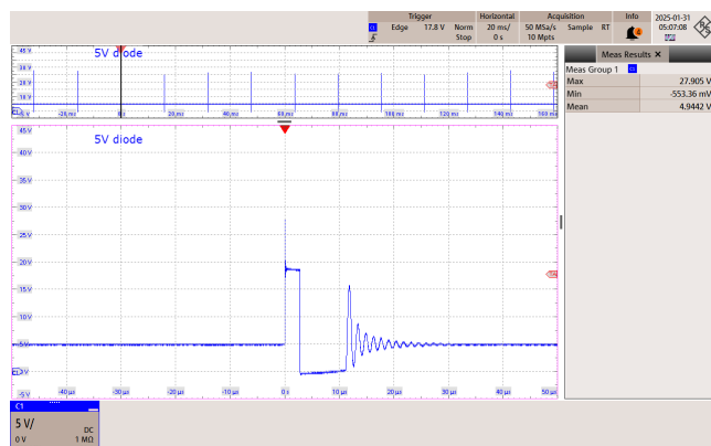
Figure 63 – 230 VAC 50 Hz.
