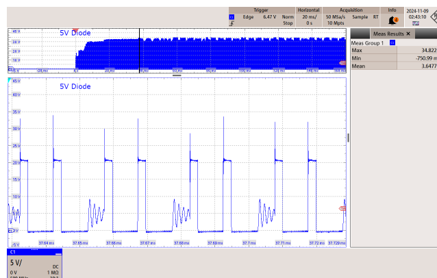
Figure 68 – 265 VAC 50 Hz.
