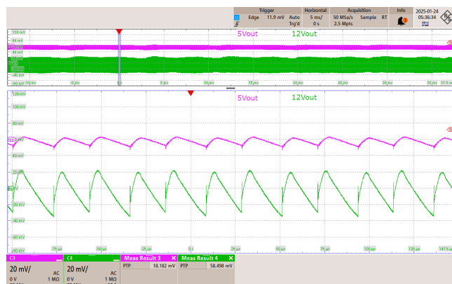
Figure 111 – 85 VAC 60 Hz.
