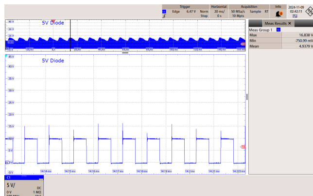
Figure 57 – 85 VAC 60 Hz.
