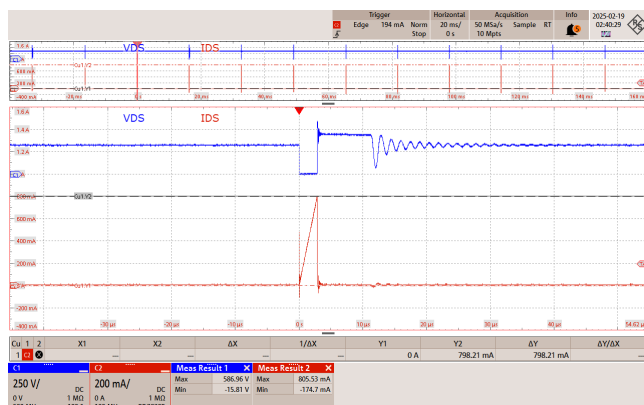
Figure 31 – 230 VAC 50 Hz.
