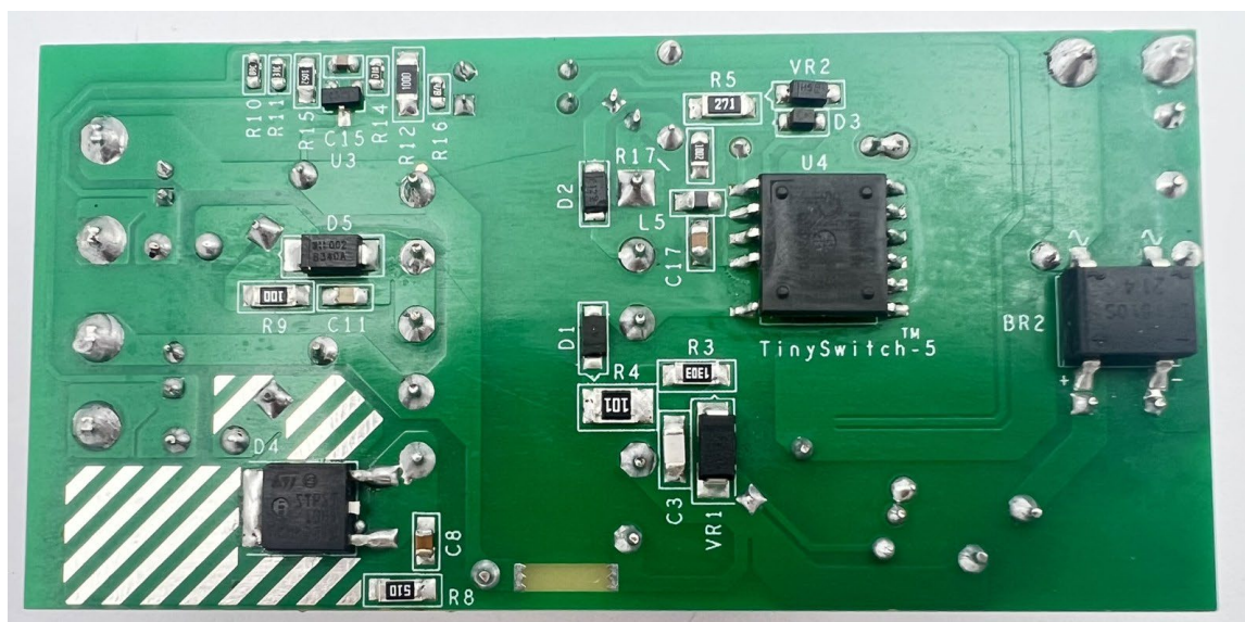
Figure 2 – Photograph, Bottom View.
