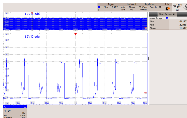
Figure 44 – 265 VAC 50 Hz.
