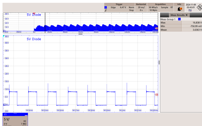
Figure 65 – 85 VAC 60 Hz.
