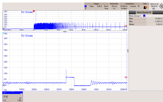
Figure 69 – 85 VAC 60 Hz.
