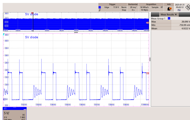
Figure 59 – 230 VAC 50 Hz.
