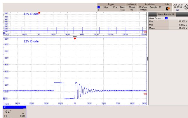
Figure 45 – 85 VAC 60 Hz.
