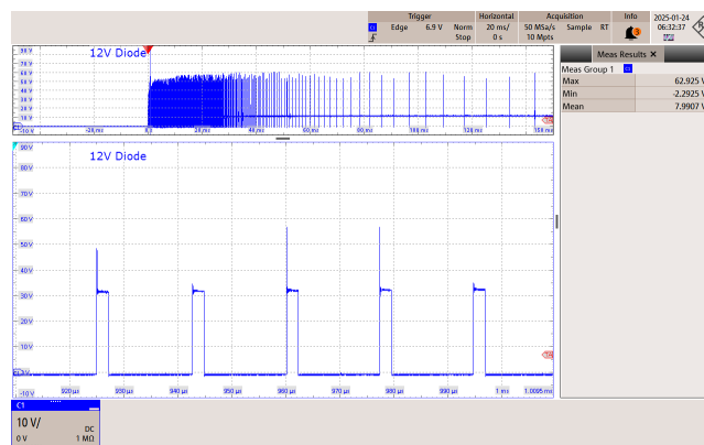
Figure 56 – 265 VAC 50 Hz.
