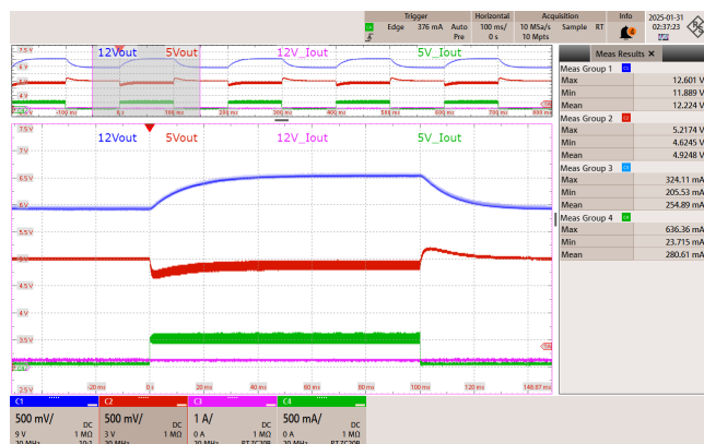
Figure 87 – 230 VAC 50 Hz.
