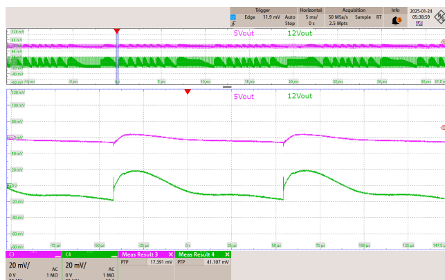
Figure 119 – 85 VAC 60 Hz.
