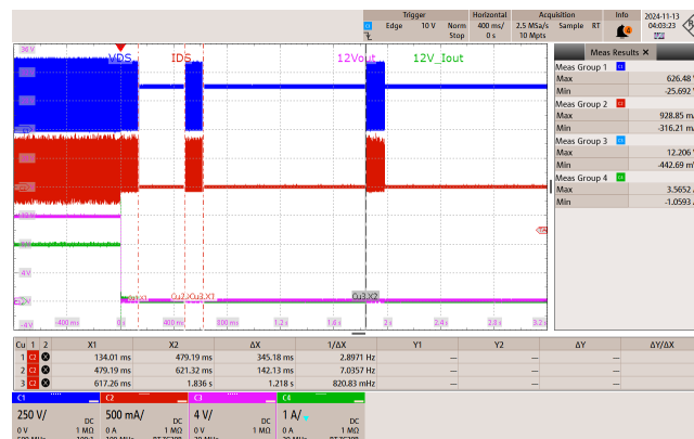
Figure 134 – 265 VAC 50 Hz. 12 V Running Output Short.
