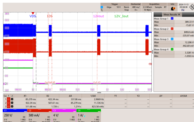
Figure 133 – 85 VAC 60 Hz 12 V Running Output Short.
