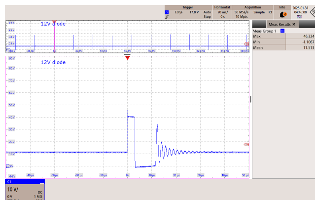
Figure 46 – 115 VAC 60 Hz.
