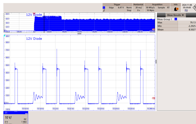
Figure 52 – 265 VAC 50 Hz.
