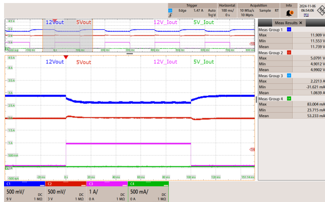
Figure 93 – 85 VAC 60 Hz.
