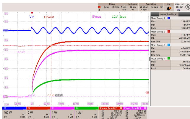
Figure 77 – 85 VAC 60 Hz.
