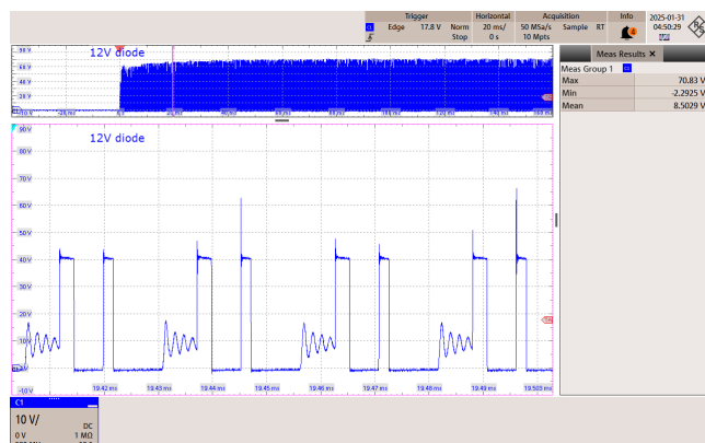
Figure 51 – 230 VAC 50 Hz.
