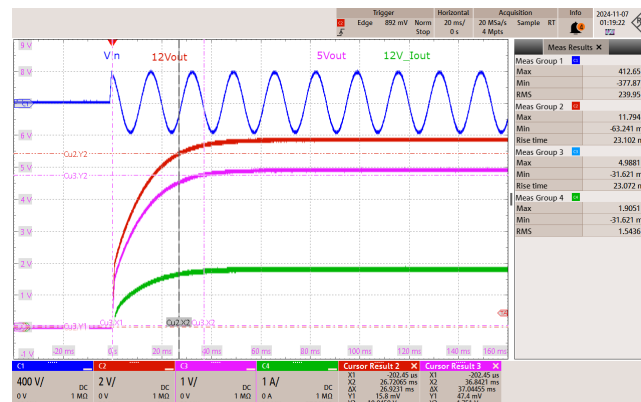
Figure 80 – 265 VAC 50 Hz.
