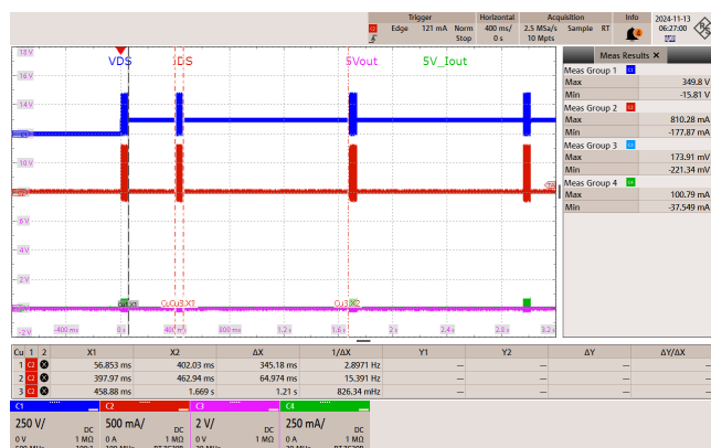
Figure 131 – 85 VAC 60 Hz 5 V Start-Up Output Short.
