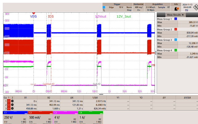
Figure 137 – 85 VAC 60 Hz 12 V / 2.3 A, 5 V / 0.575 A.
