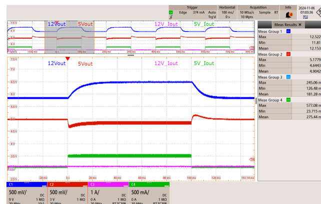
Figure 88 – 265 VAC 50 Hz.
