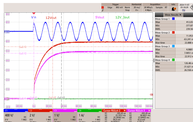
Figure 84 – 265 VAC 50 Hz.
