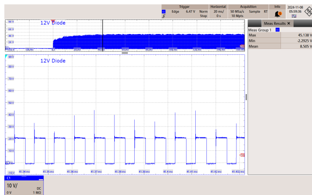
Figure 49 – 85 VAC 60 Hz.
