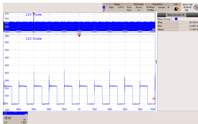
Figure 41 – 85 VAC 60 Hz.
