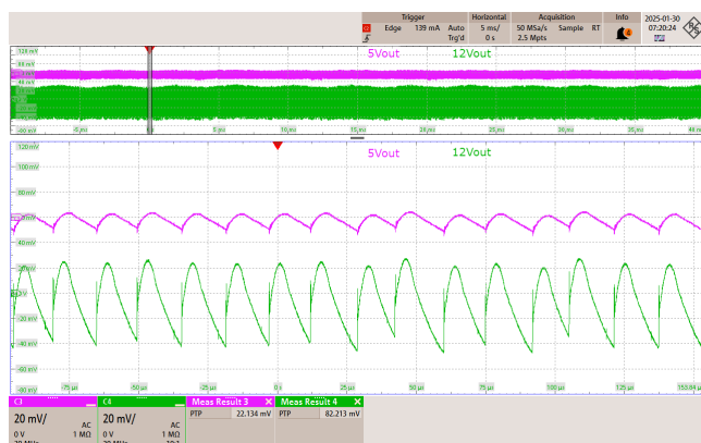
Figure 109 – 230 VAC 50 Hz.
