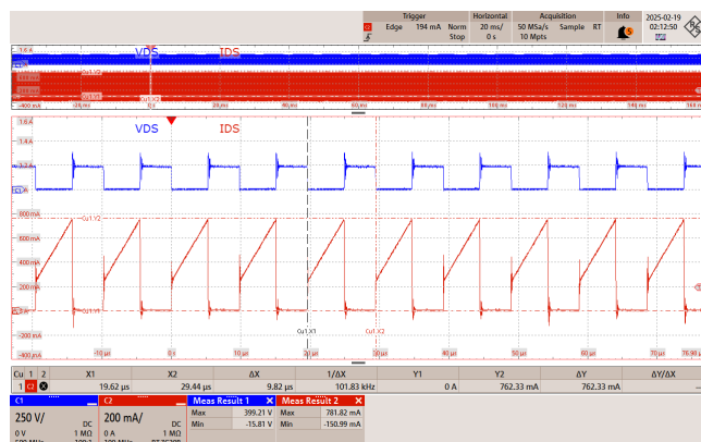
Figure 25 – 85 VAC 60 Hz.
