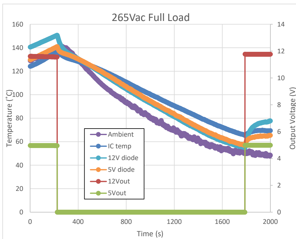
Figure 140 – 265 VAC 50 Hz Full Load OTP.
