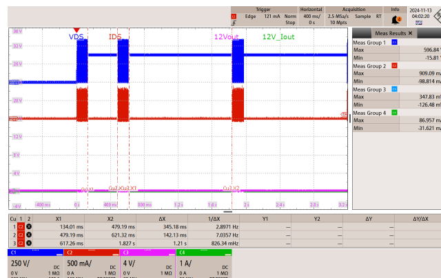
Figure 130 – 265 VAC 50 Hz 12 V Start-Up Output Short.
