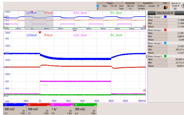
Figure 94 – 115 VAC 60 Hz.
