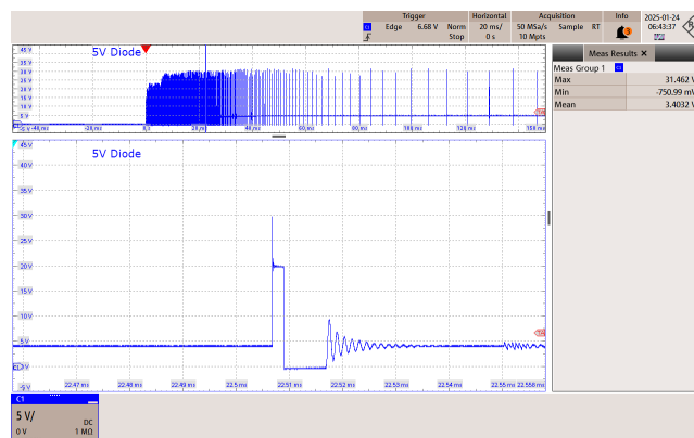
Figure 72 – 265 VAC 50 Hz.
