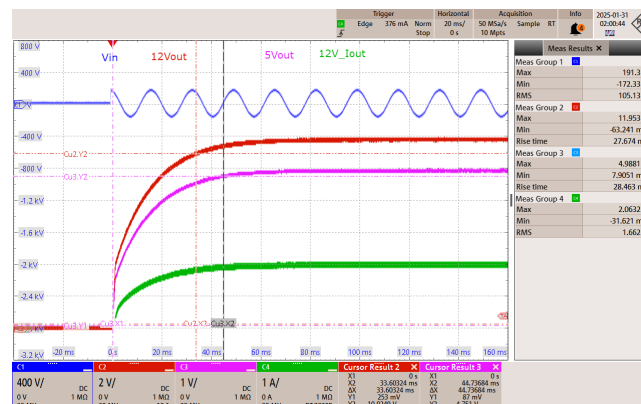
Figure 78 – 115 VAC 60 Hz.
