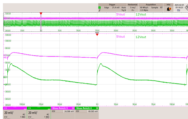
Figure 122 – 265 VAC 50 Hz.
