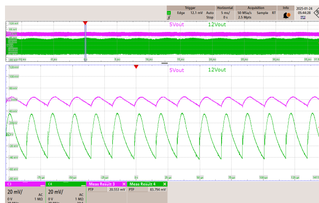
Figure 110 – 265 VAC 50 Hz.
