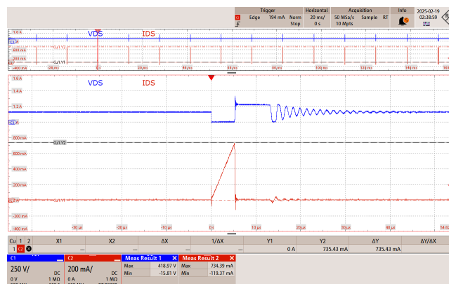
Figure 30 – 115 VAC 60 Hz.
