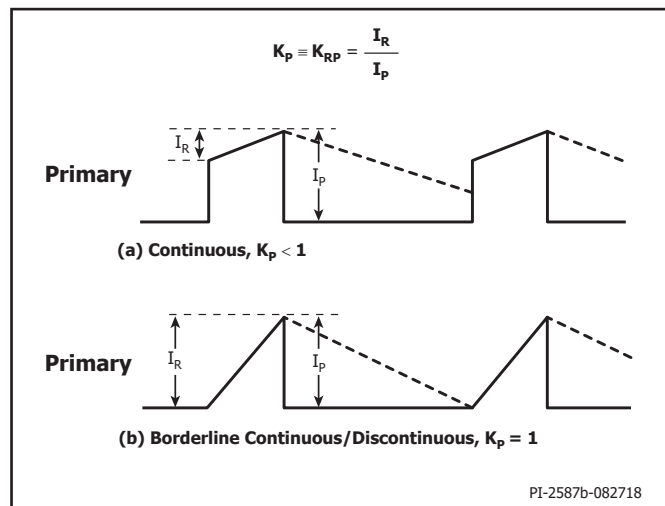
Figure 13. Continuous Conduction Mode Current Waveform, K_p < 1 .
